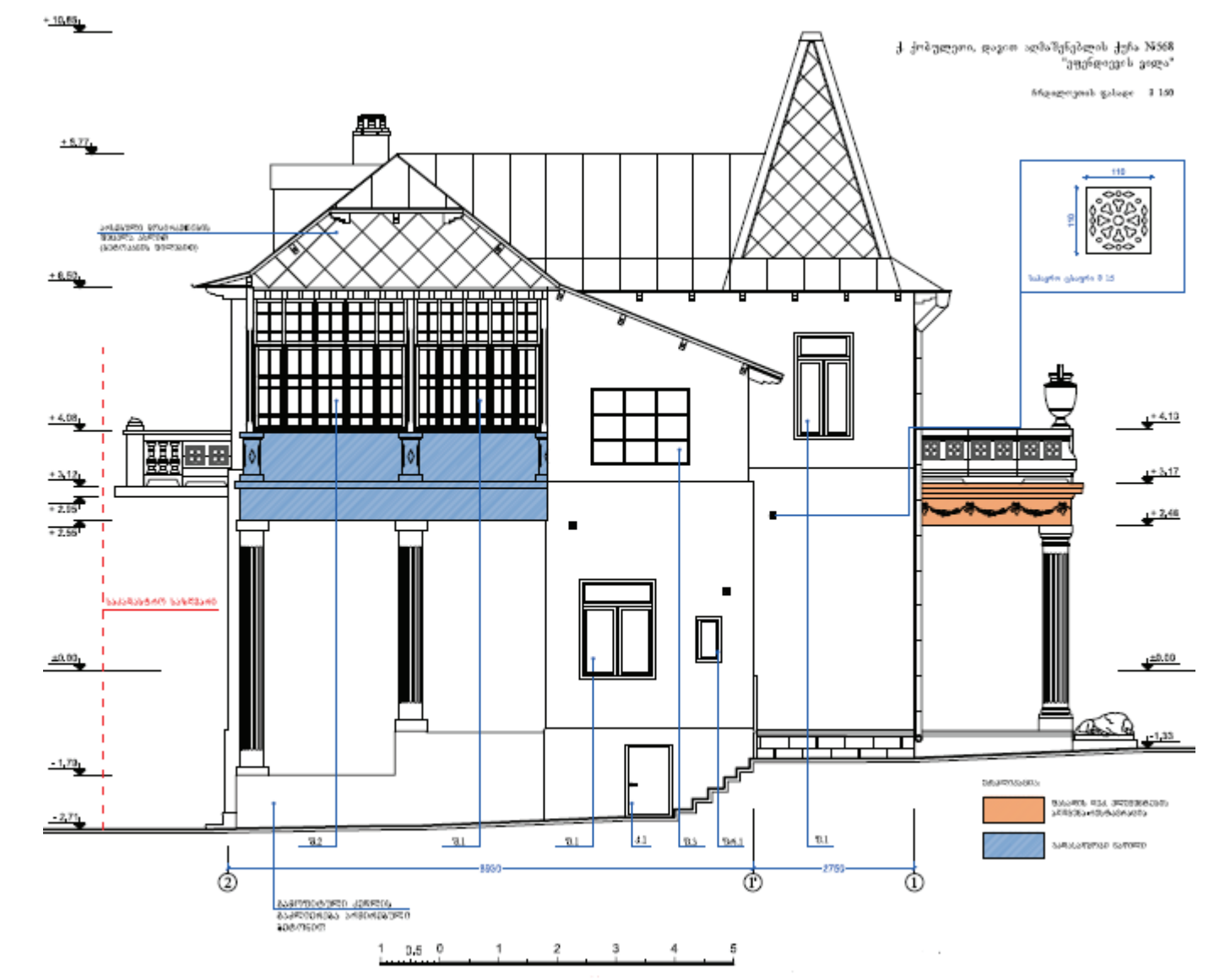
NORTH ELEVATION
