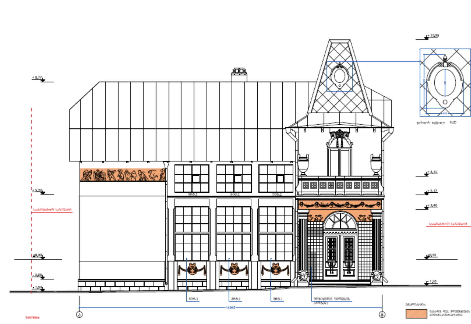
WEST ELEVATION
